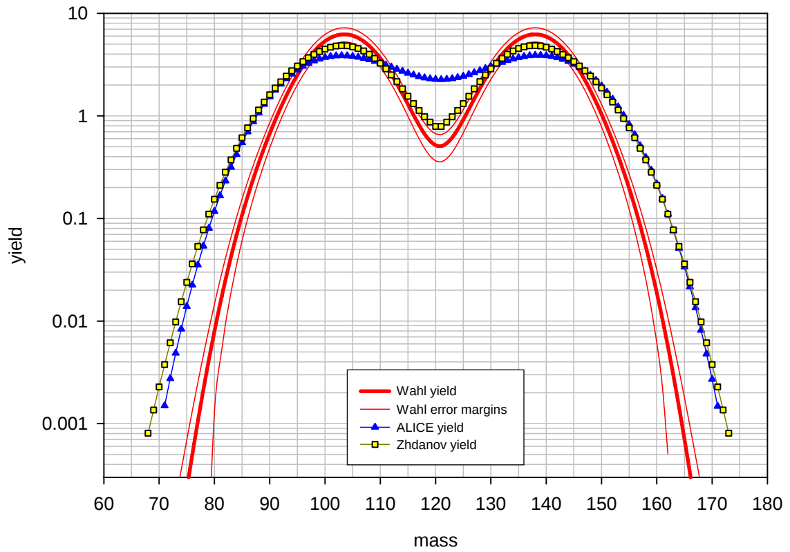
Benchmark B: ^{241}\text{Am} at 13 MeV, pre-neutron emission mass distribution
